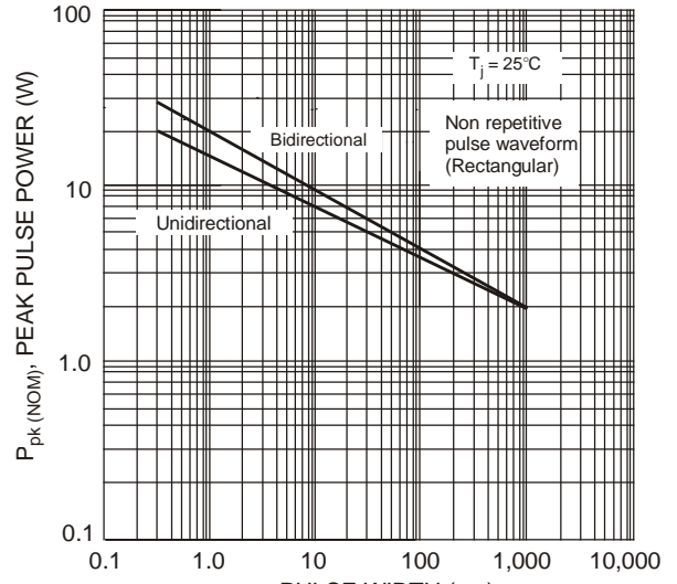
Fig. 8 Pulse Rating Curve, P_{pk(NOM)} (W) vs. Pulse Width (ms) Power is defined as P_{pk(NOM)} = V_{BR(NOM)} \times I_{pp} where V_{BR(NOM)} is the nominal breakdown voltage
