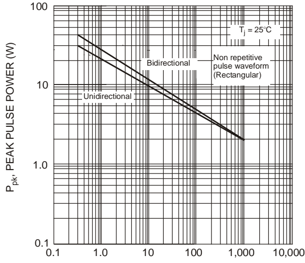
Fig. 7 Pulse Rating Curve, P_{pk} (W) vs. Pulse Width (ms) Power is defined as P_{pk} = V_C \times I_{pp}
